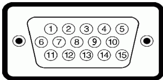
Pin 15-pin Side of the Connected Signal Number Cable
